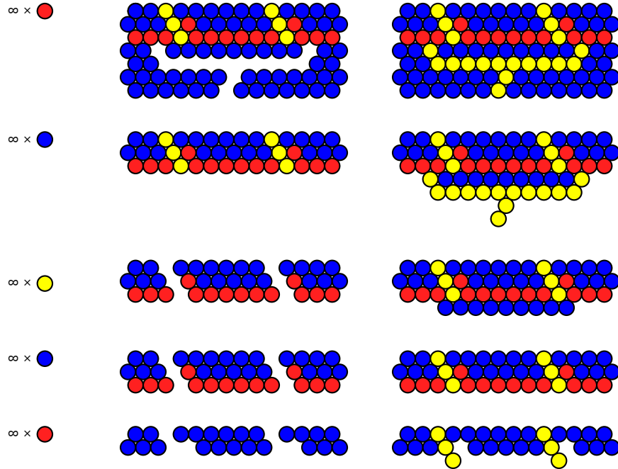
Fig. 3. Split gadget. (Left) Behavior of a chosen set. (Right) Behavior of an unchosen set.
