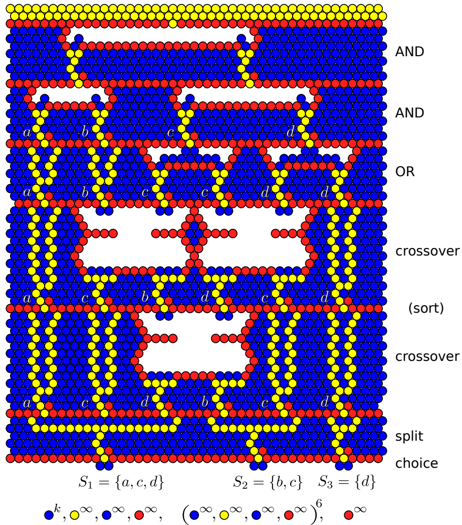
Fig. 7. Example of the main construction (the gray box in Figure 1) with three sets and four elements. The bubble sequence at the bottom can solve the puzzle for k = 2 and k = 3 , but not for k = 1 .
