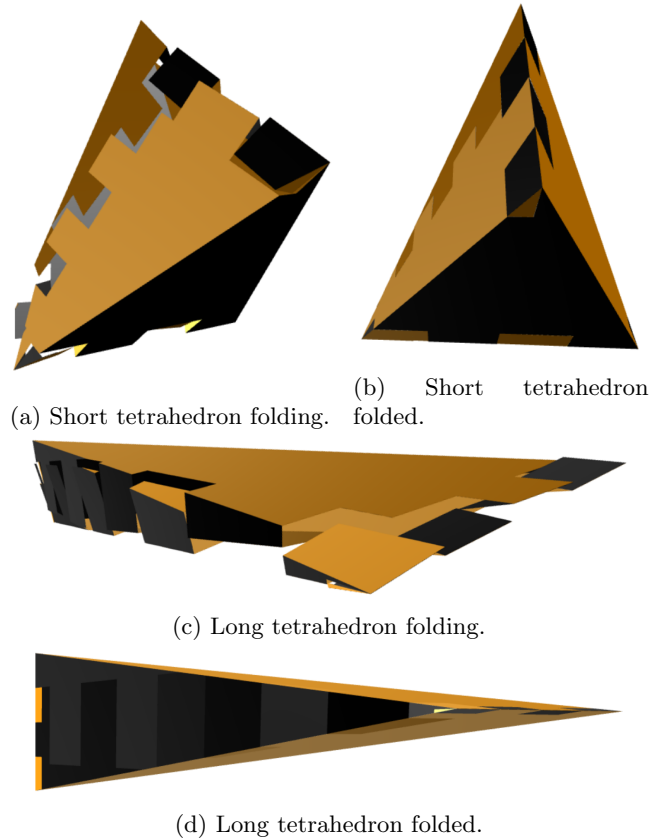
Figure 9: Folding tetrahedra
