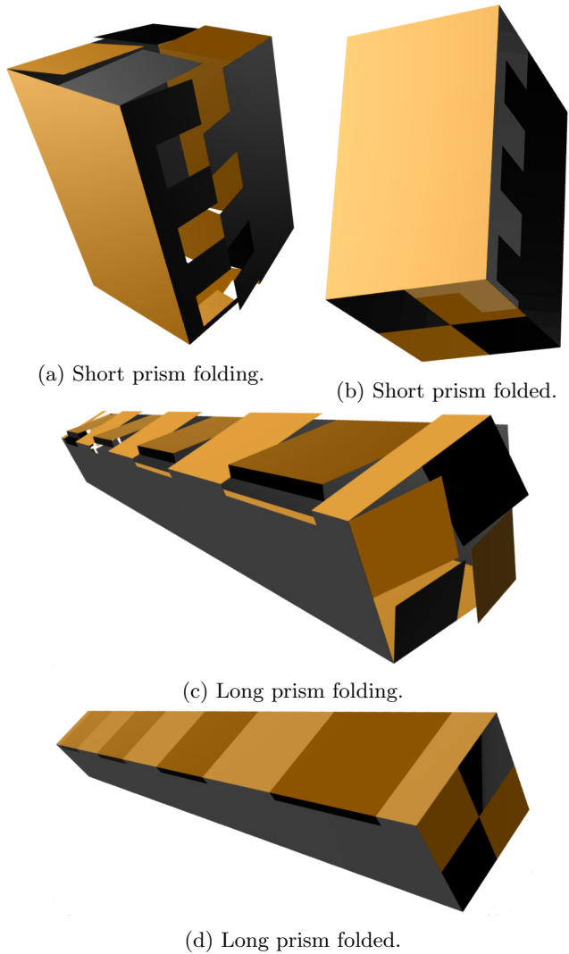
Figure 6: Two different square prisms from a common development.
