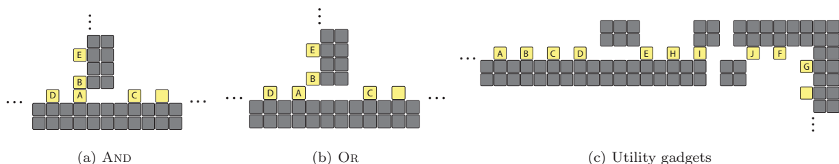
Figure 15: Sokoban gadgets.
