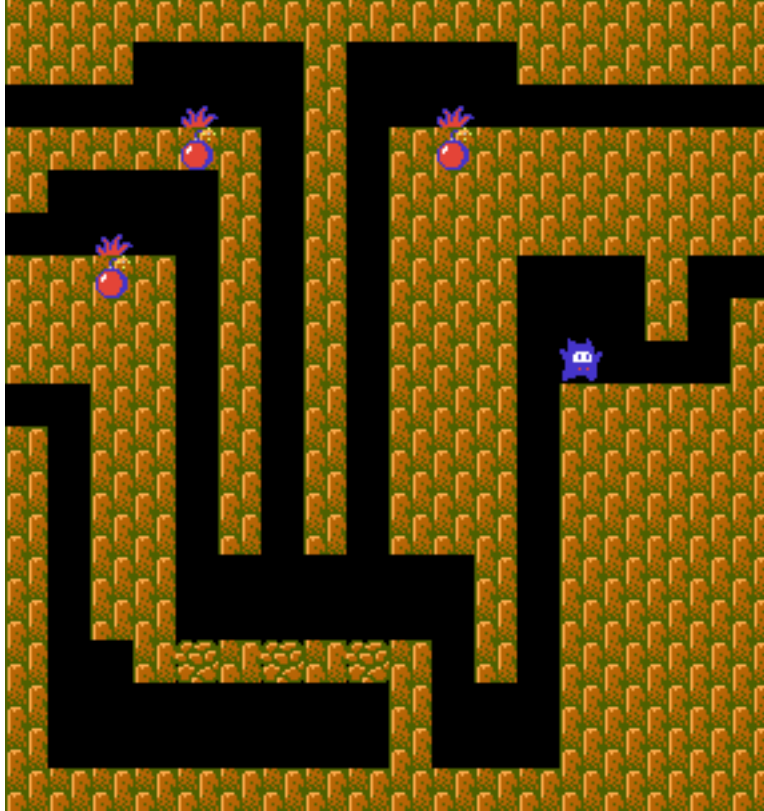
Figure 16: Clause gadget for American SMB 2
